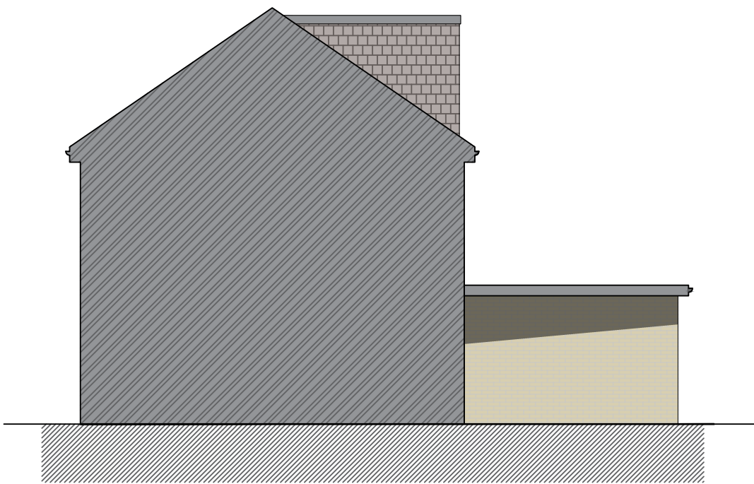
Proposed Side Elevation 1:50
