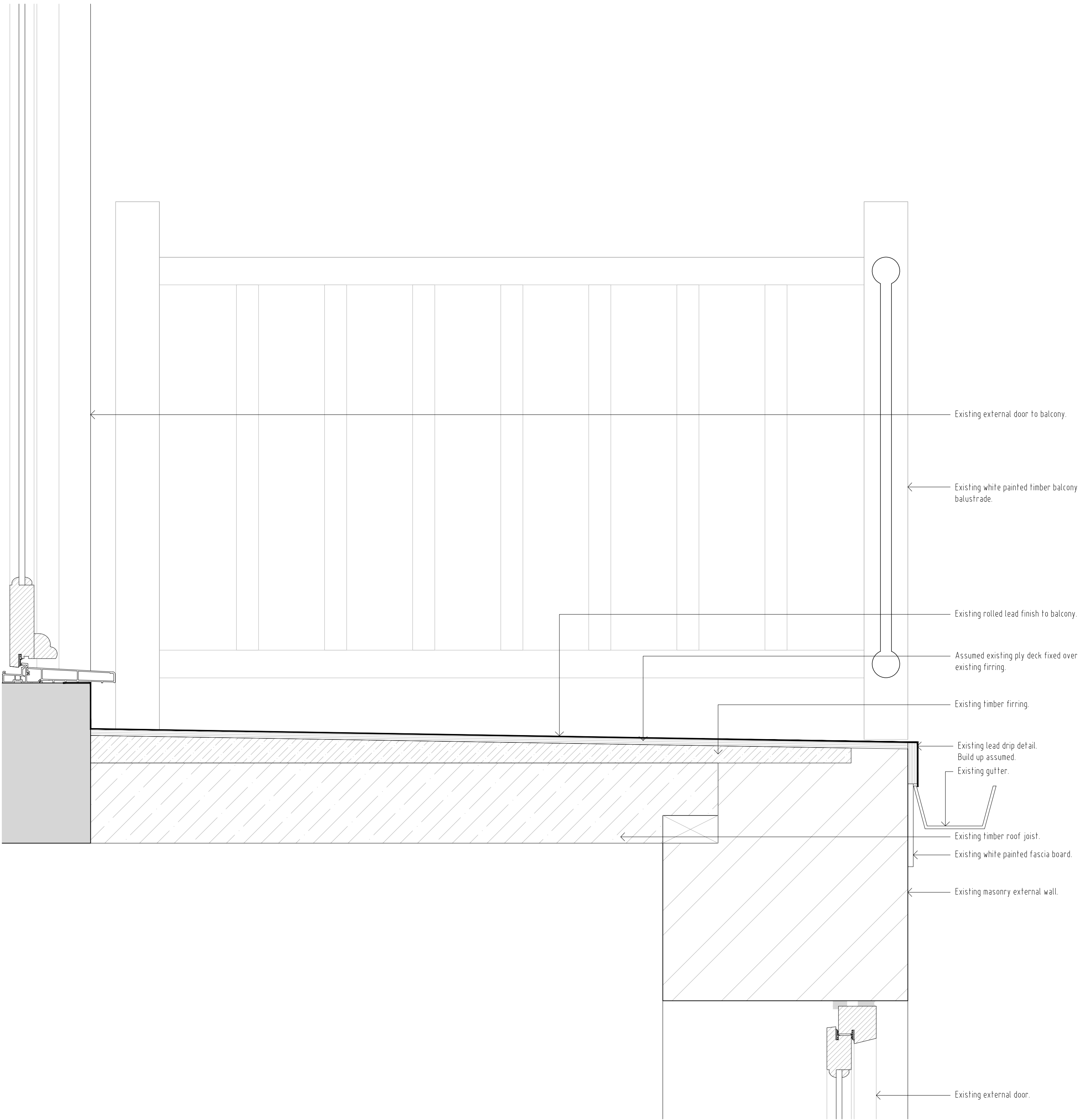
Existing Boathouse Balcony Section Detail
