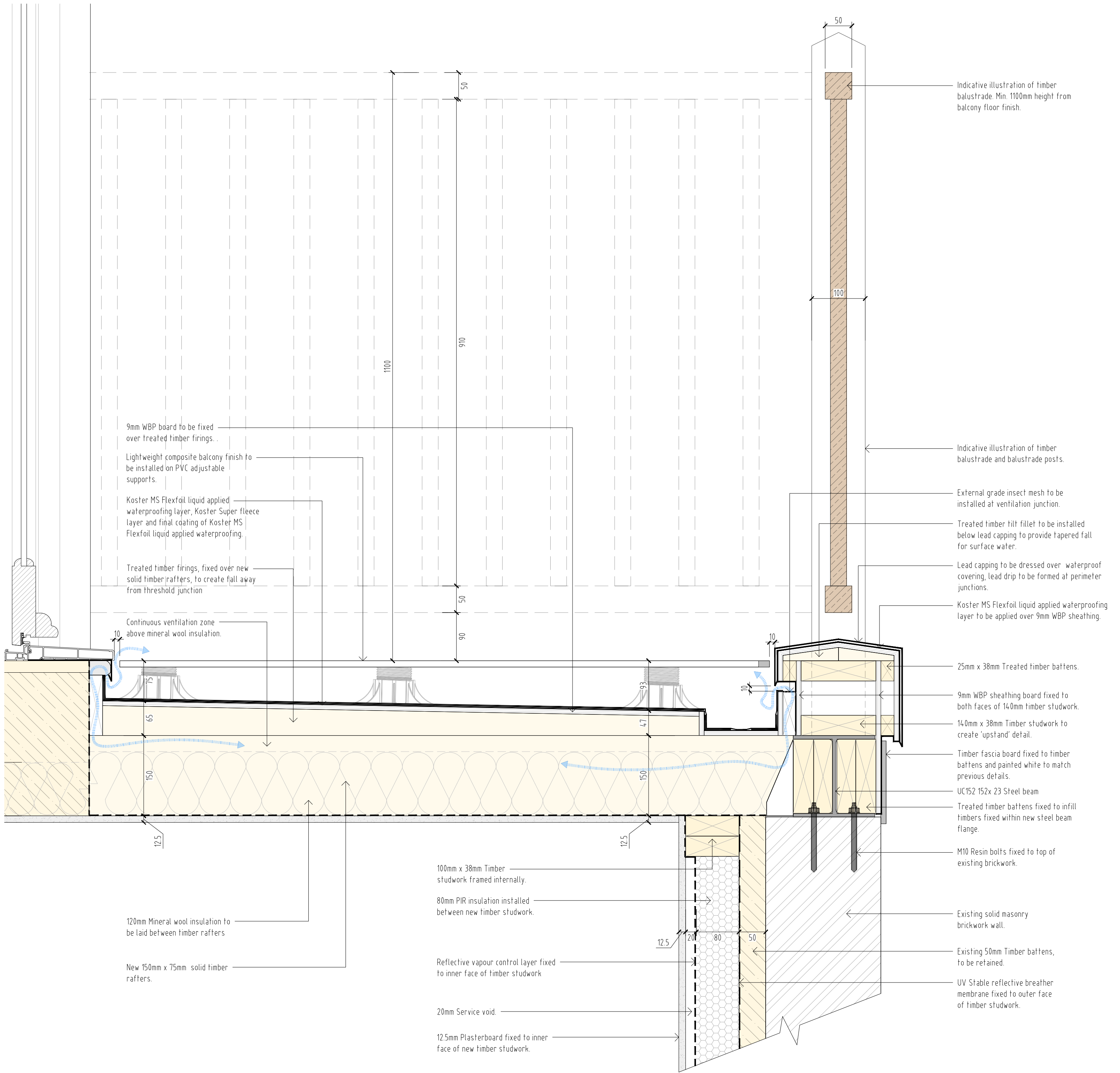
Proposed Boathouse Balcony Section Detail
