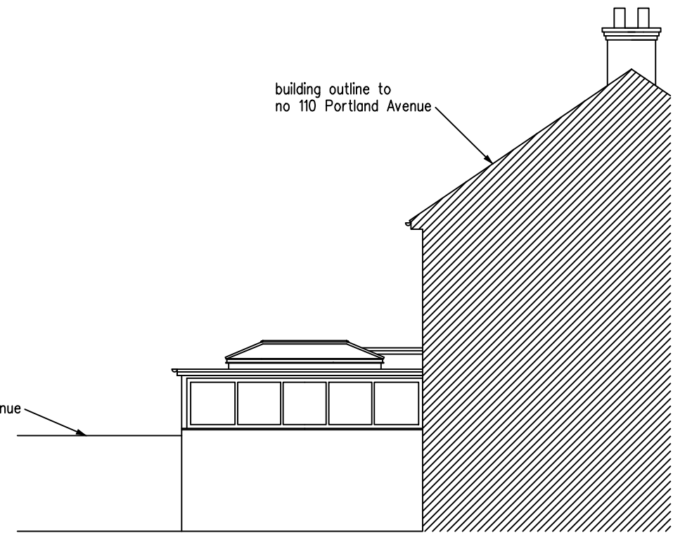
EXISTING SIDE ELEVATION (FACING NO.110)
