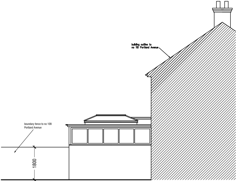
PROPOSED SIDE ELEVATION (FACING NO.110) Scale 1:100
