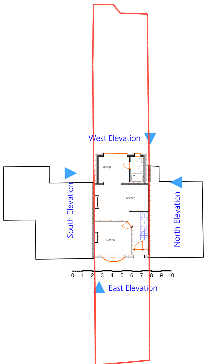
3 Site Plan Proposed 1:200
