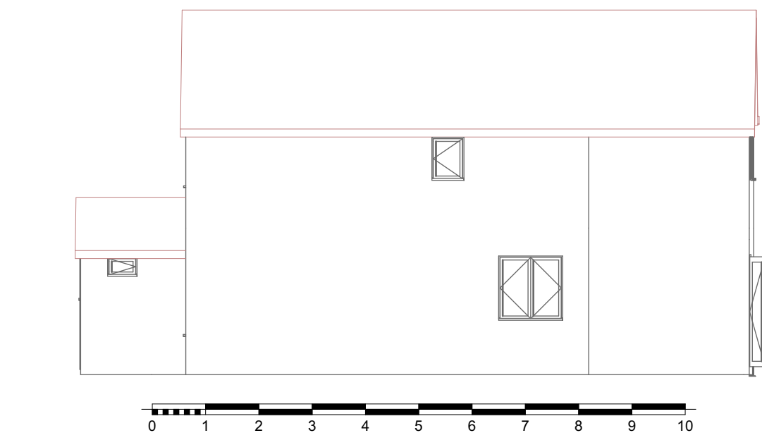
9 West Elevation Proposed 1:100
