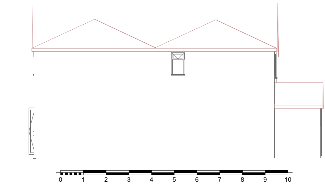
8 East Elevation Proposed 1:100
