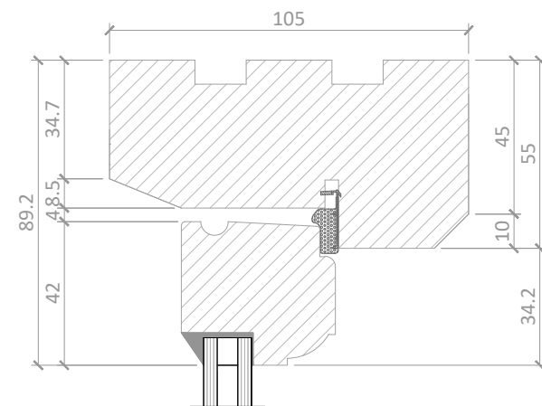
DETAIL 4
