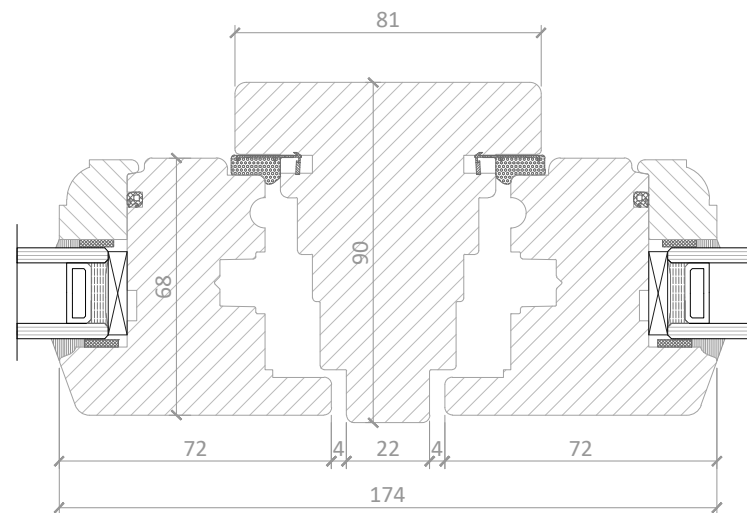
DETAIL 2
