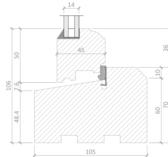
DETAIL 5
