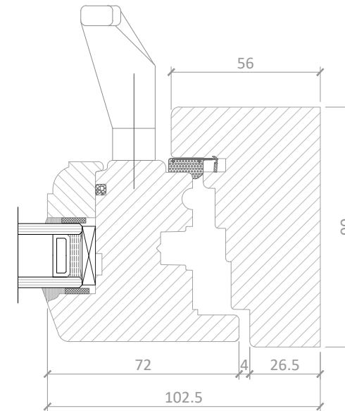
DETAIL 3
