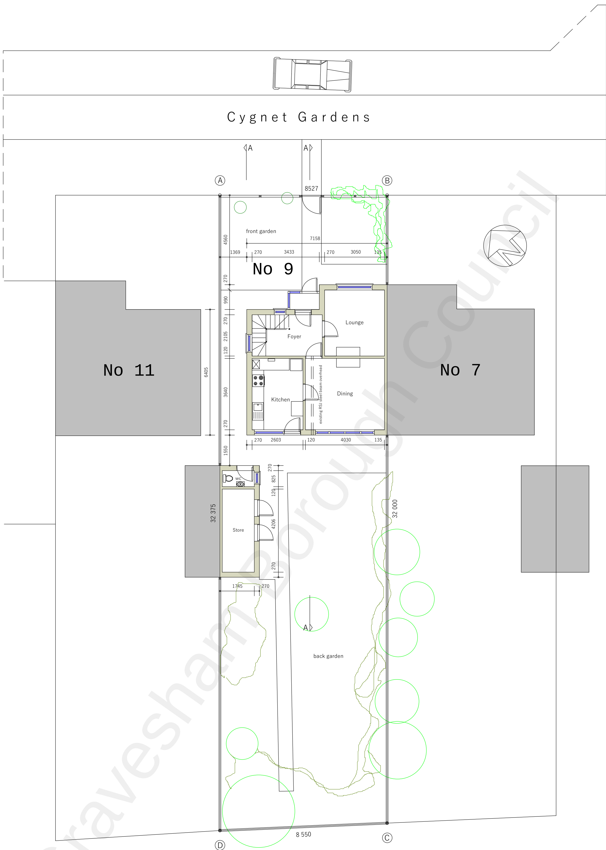
0 Existing Ground Floor Plan
