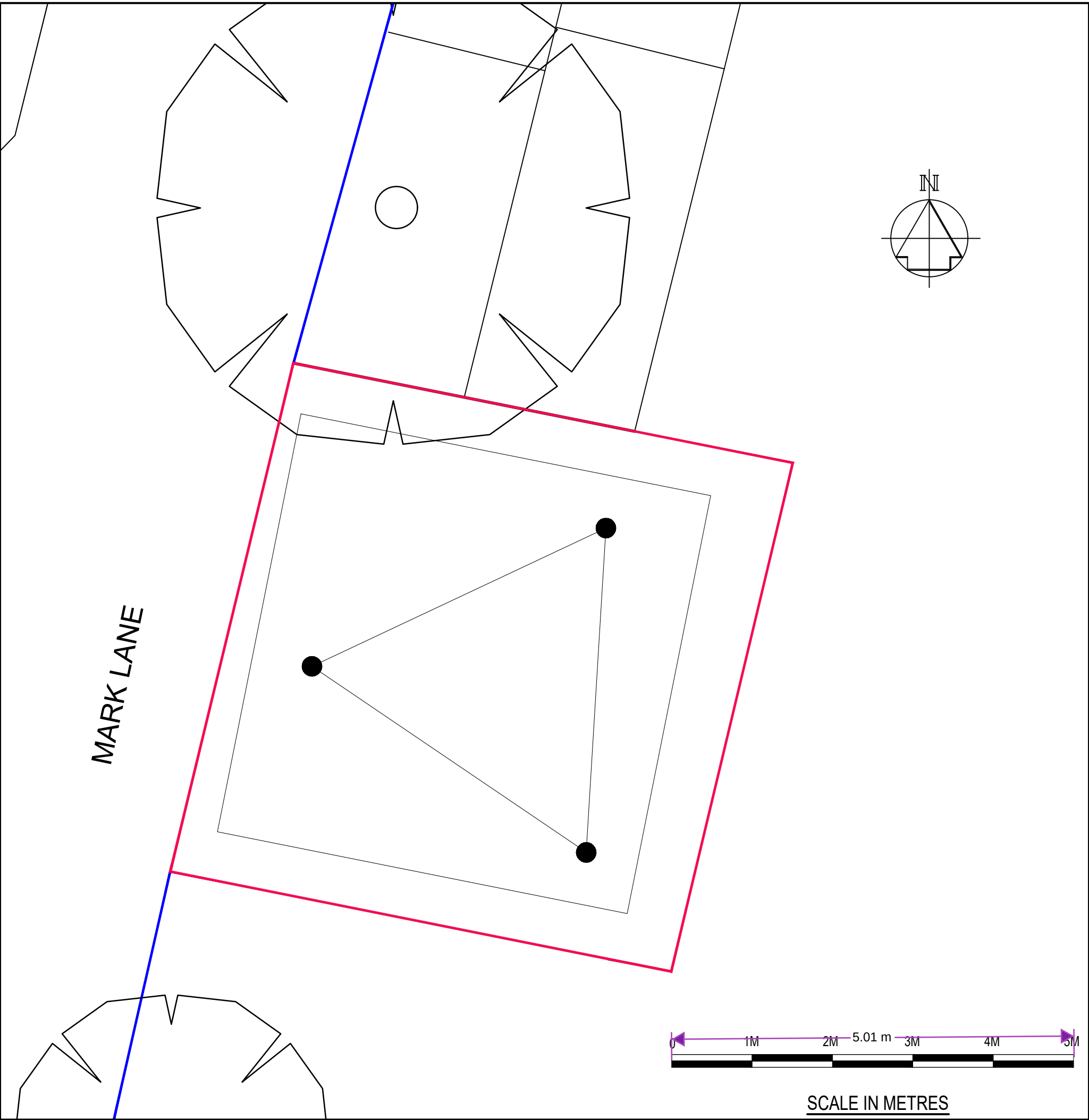
EXISTING RADAR TOWER BASE PLAN (1:50)
