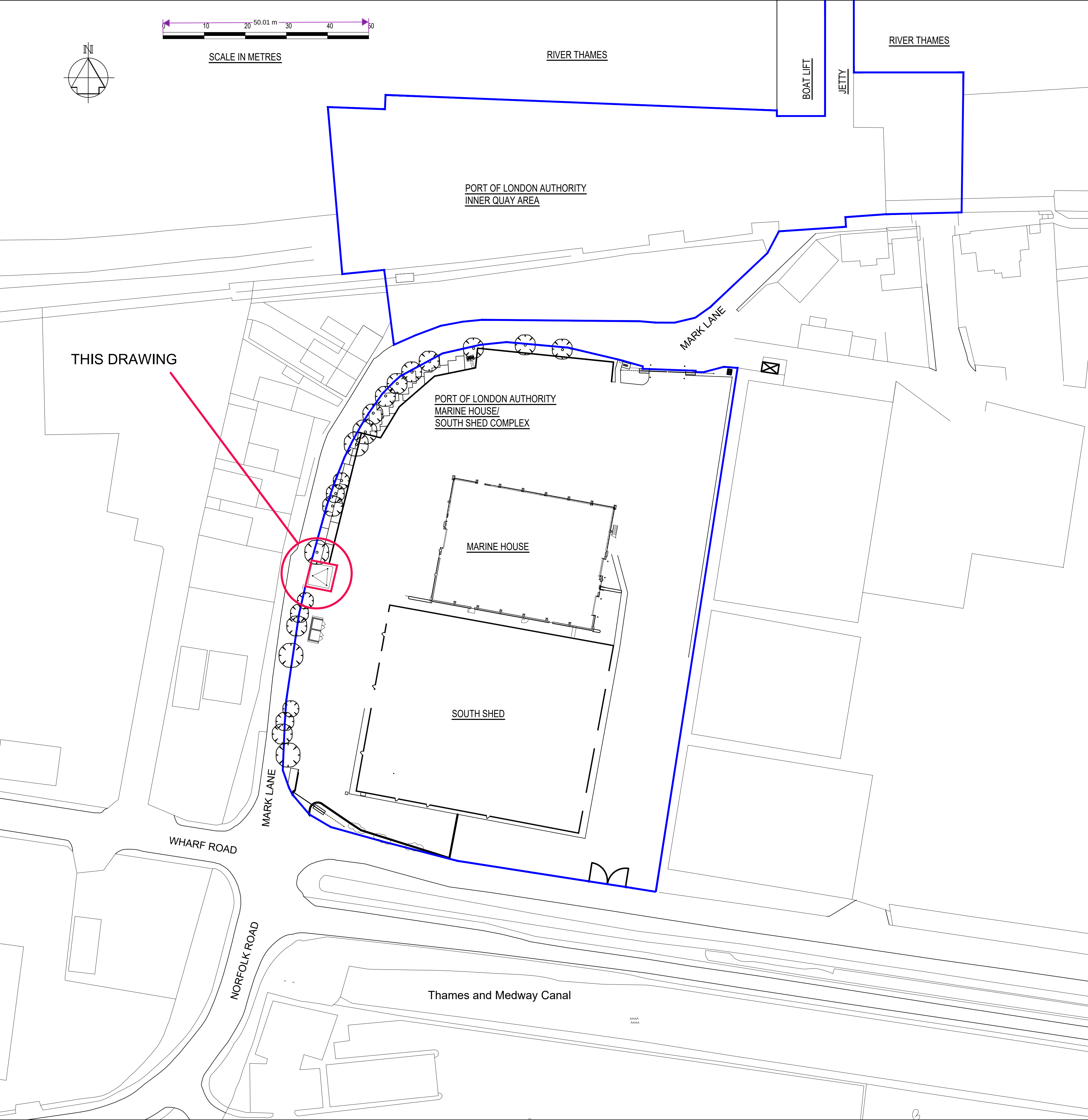
KEY PLAN (1:500)
