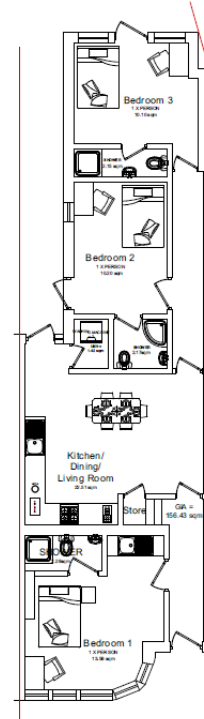
PROPOSED GROUND FLOOR PLAN
