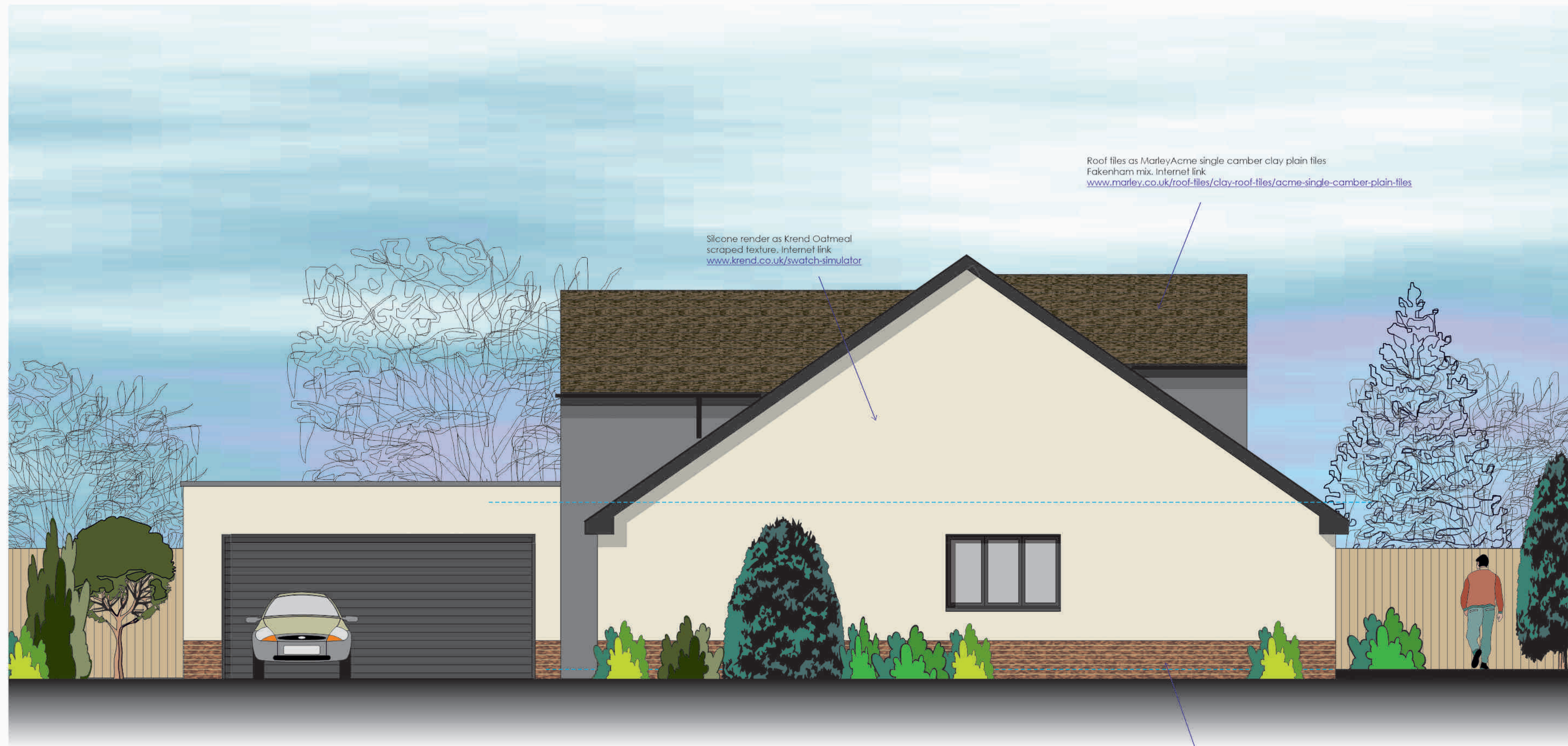
Proposed Side Elevation -1:50 EAST VIEW from FERDAGRE
