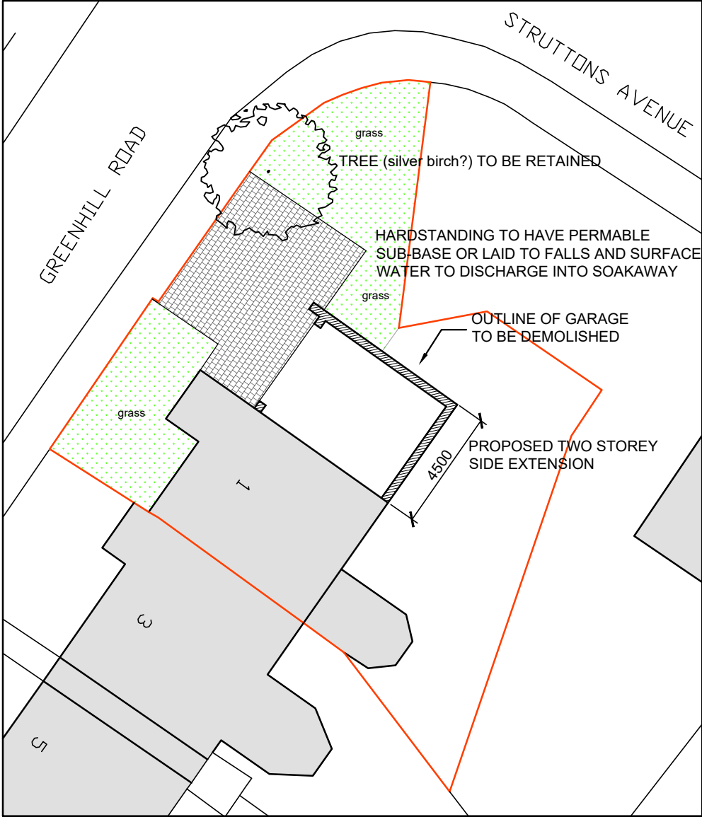
BLOCK PLAN AS PROPOSED (1:200)
