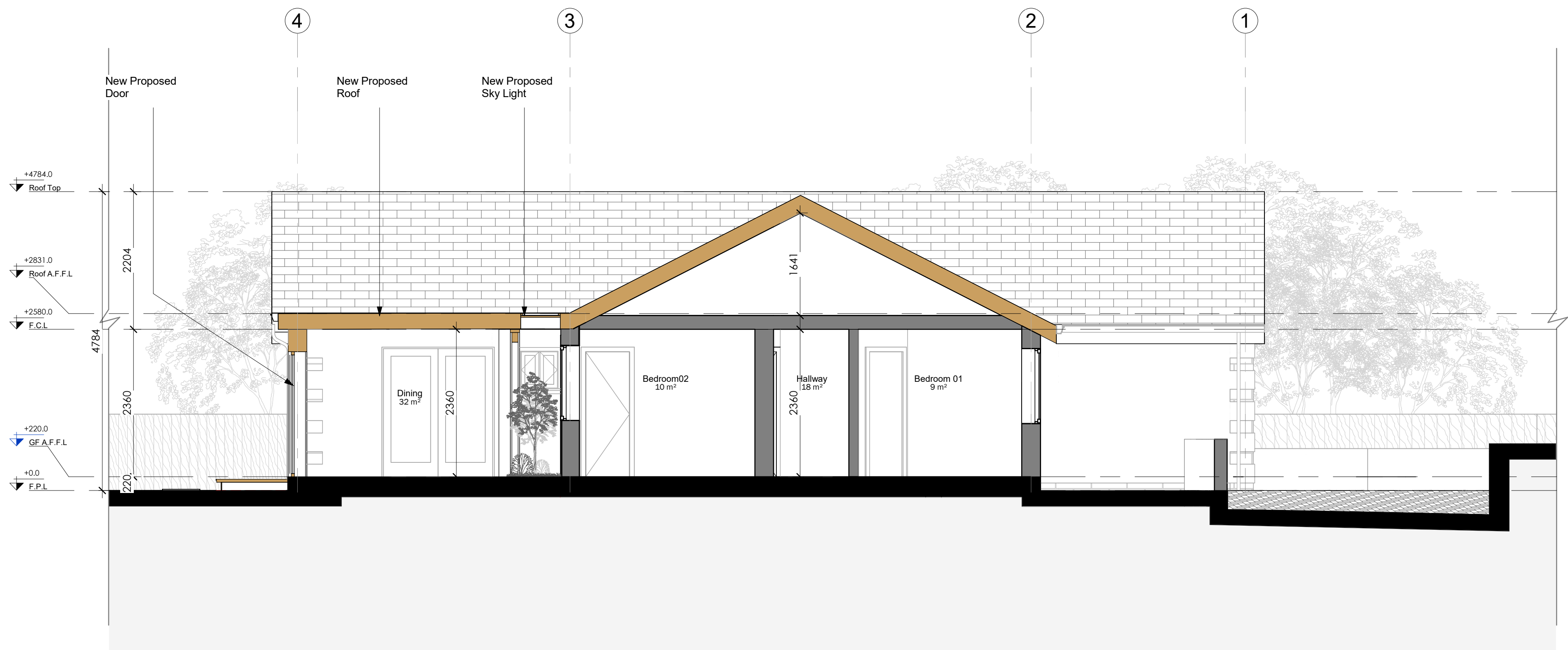
A Proposed Section A-A 311 1 : 50
