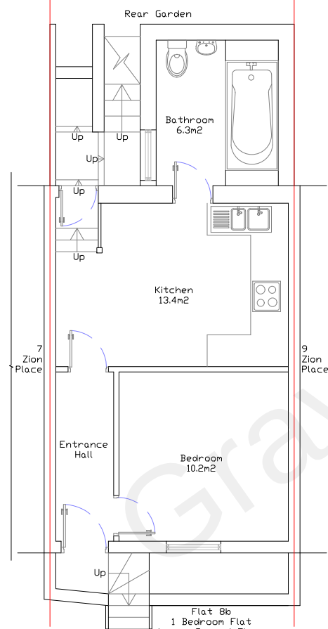
PROPOSED LOWER GROUND FLOOR PLAN
