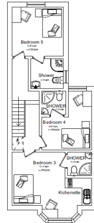
PROPOSED FIRST FLOOR PLAN
