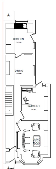
EXISTING GROUND FLOOR PLAN
