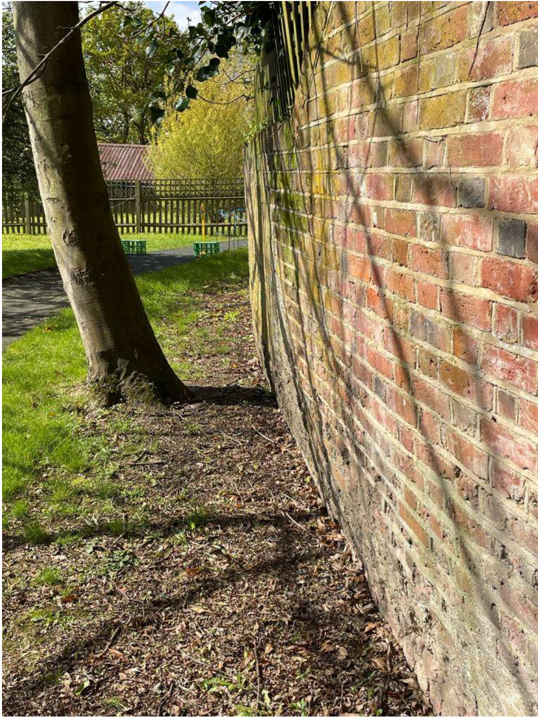
View on wall looking to south showing outward lean to wall
