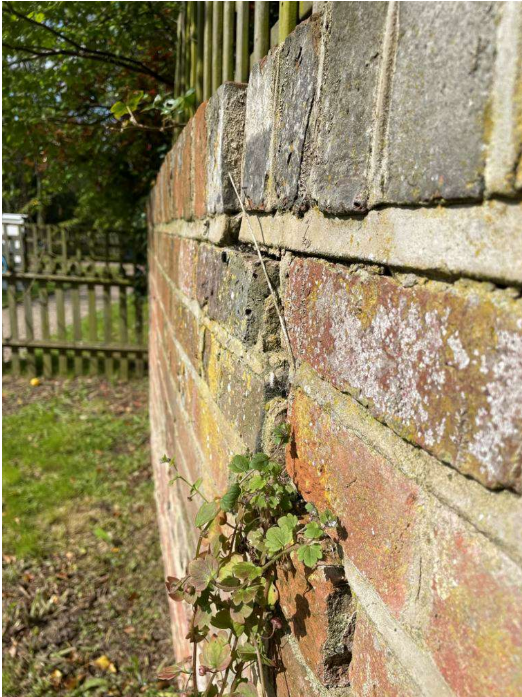
Angled view on wall showing lateral movement at vertical crack
