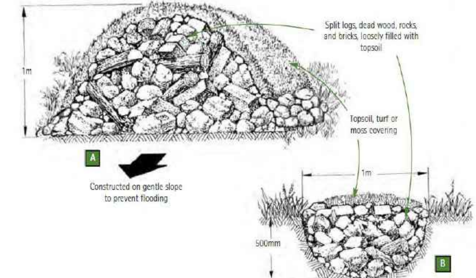
Typical Detail Of Hibernacula Design ('A' for impermeable 'B' = free draining soils)
