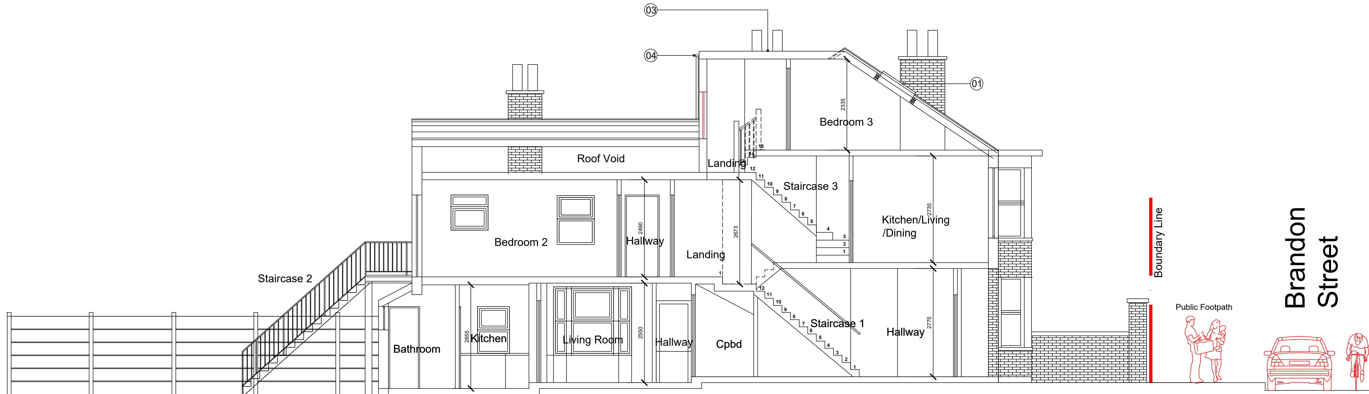
No 36 Brandon Street Proposed Section A-A
