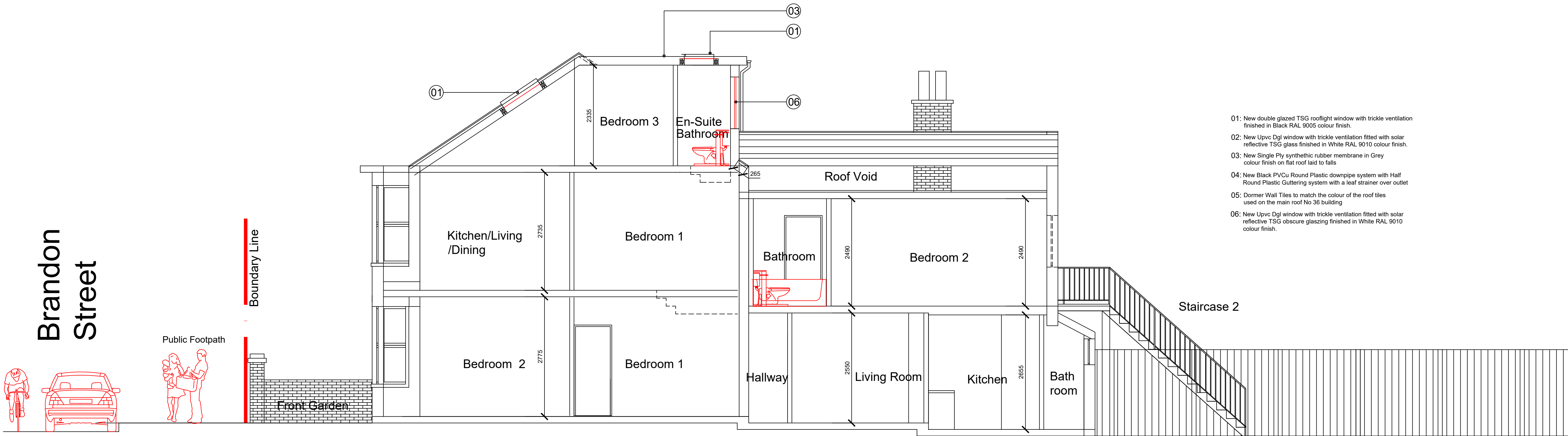
No 36 Brandon Street Proposed Section B-B
