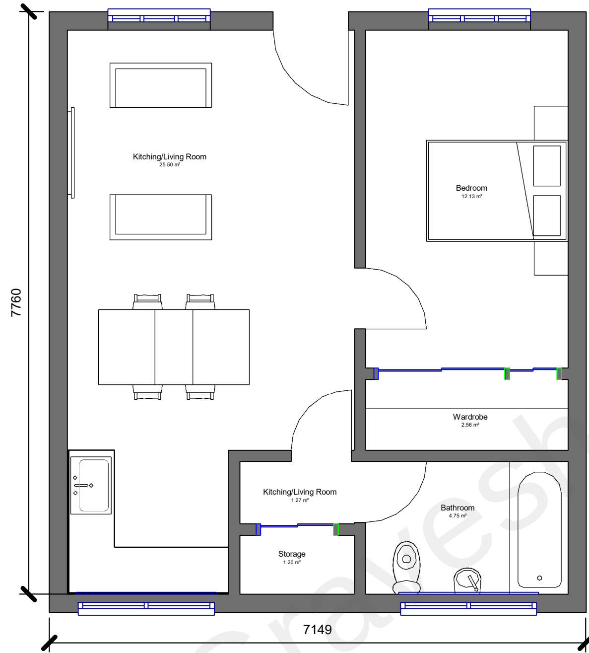
1 Proposed Ground Floor Plan 1 : 50
