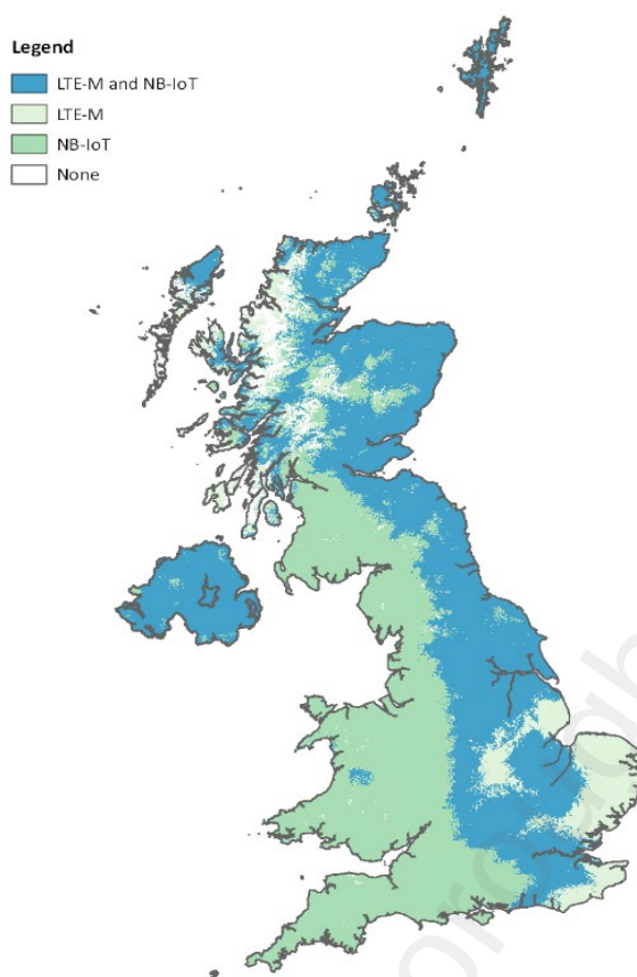
Figure 23: Map of the UK showing LTE-M and NB-IoT Coverage
