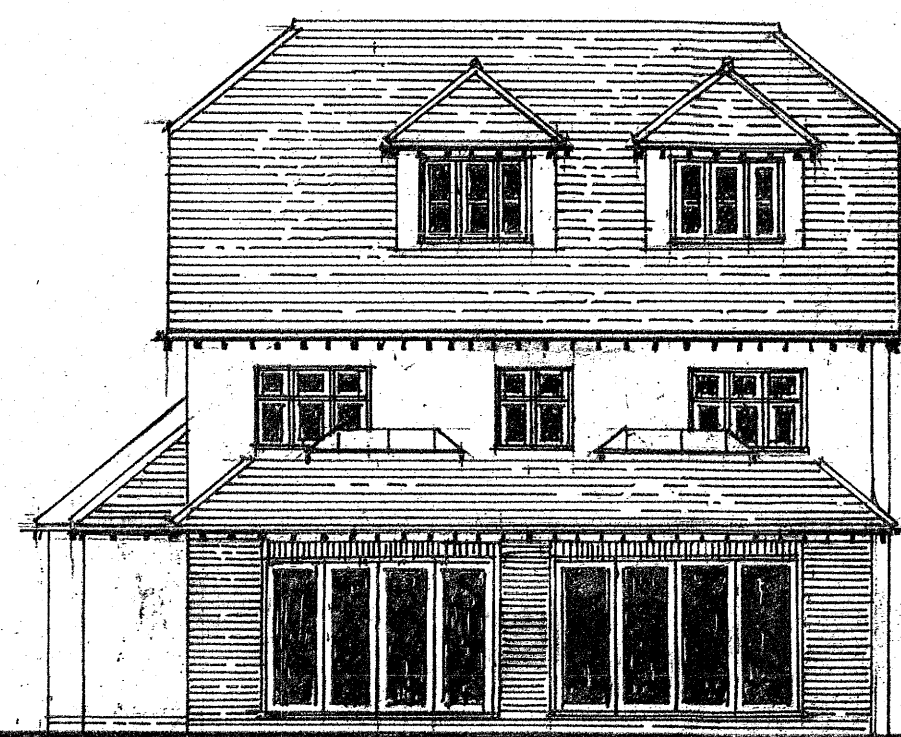
REAR ELEVATION
