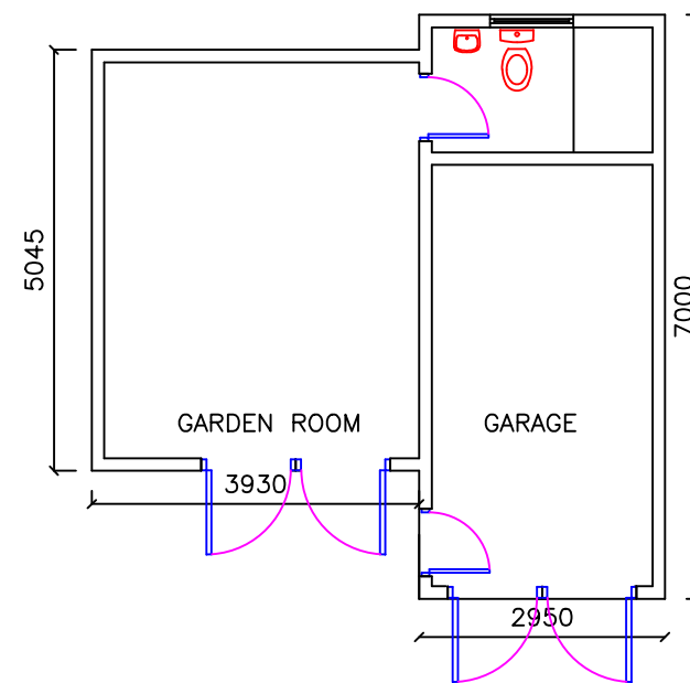
PROPOSED GARDEN ROOM AND GARAGE
