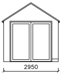
EXISTING GARAGE FRONT ELEVATION
