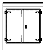
METER CABINET ELEVATION A - SOUTH WEST SCALE - 1:50
