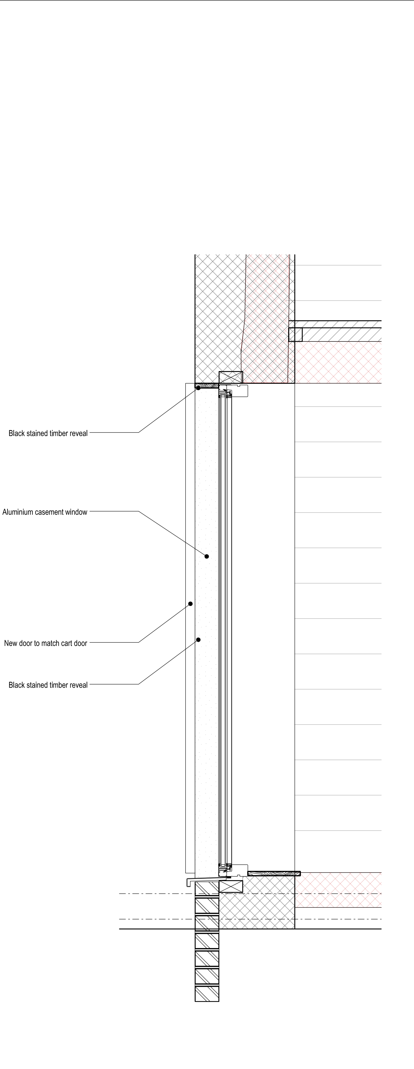
01 SECTION DETAIL
