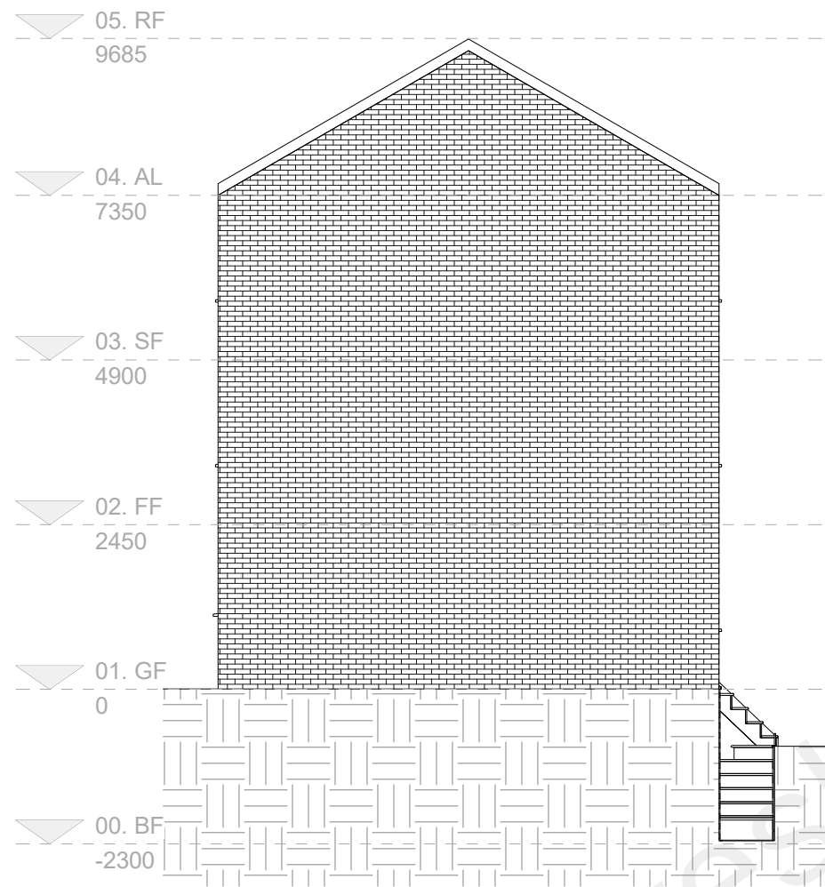
03. Right Elevation Existing 1 : 100
