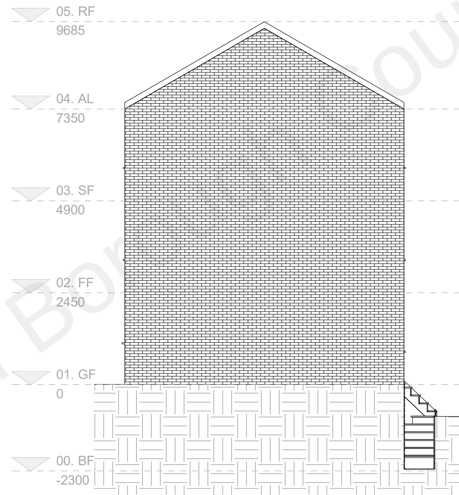
03. Right Elevation Proposed 1 : 100
