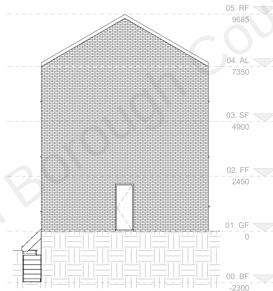
04. Left Elevation Proposed 1 : 100
