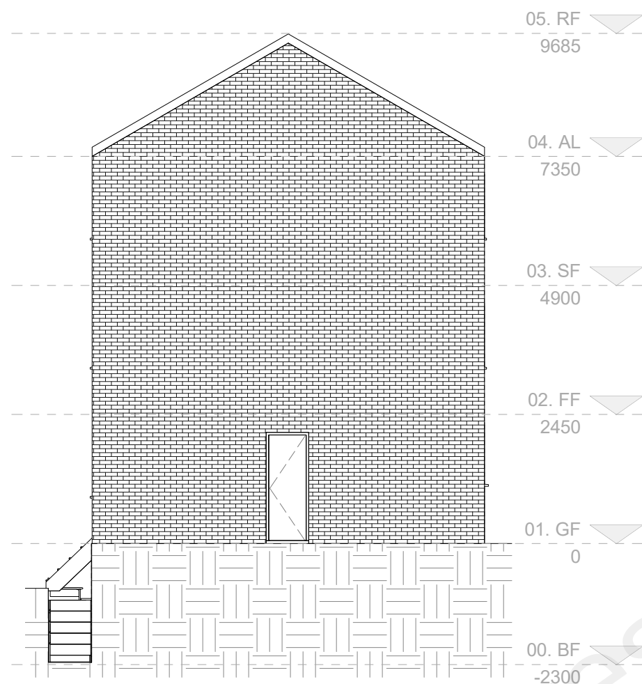
04. Left Elevation Existing 1 : 100
