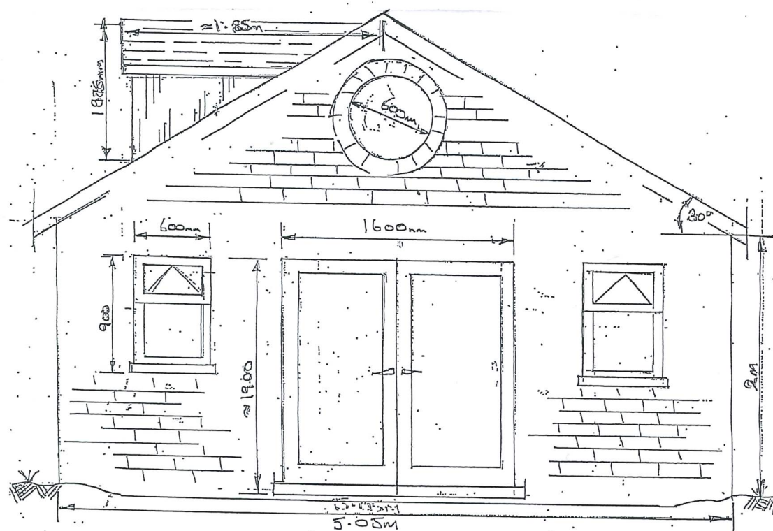
PROPOSED SIDE.
