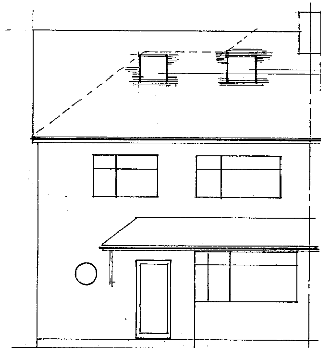
PROPOSED FRONT ELEVATION 1:100
