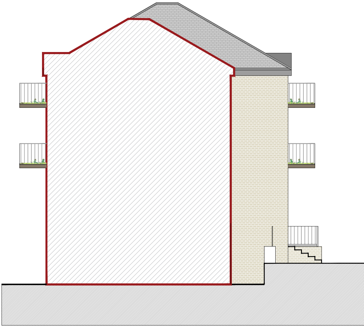
East Elevation
