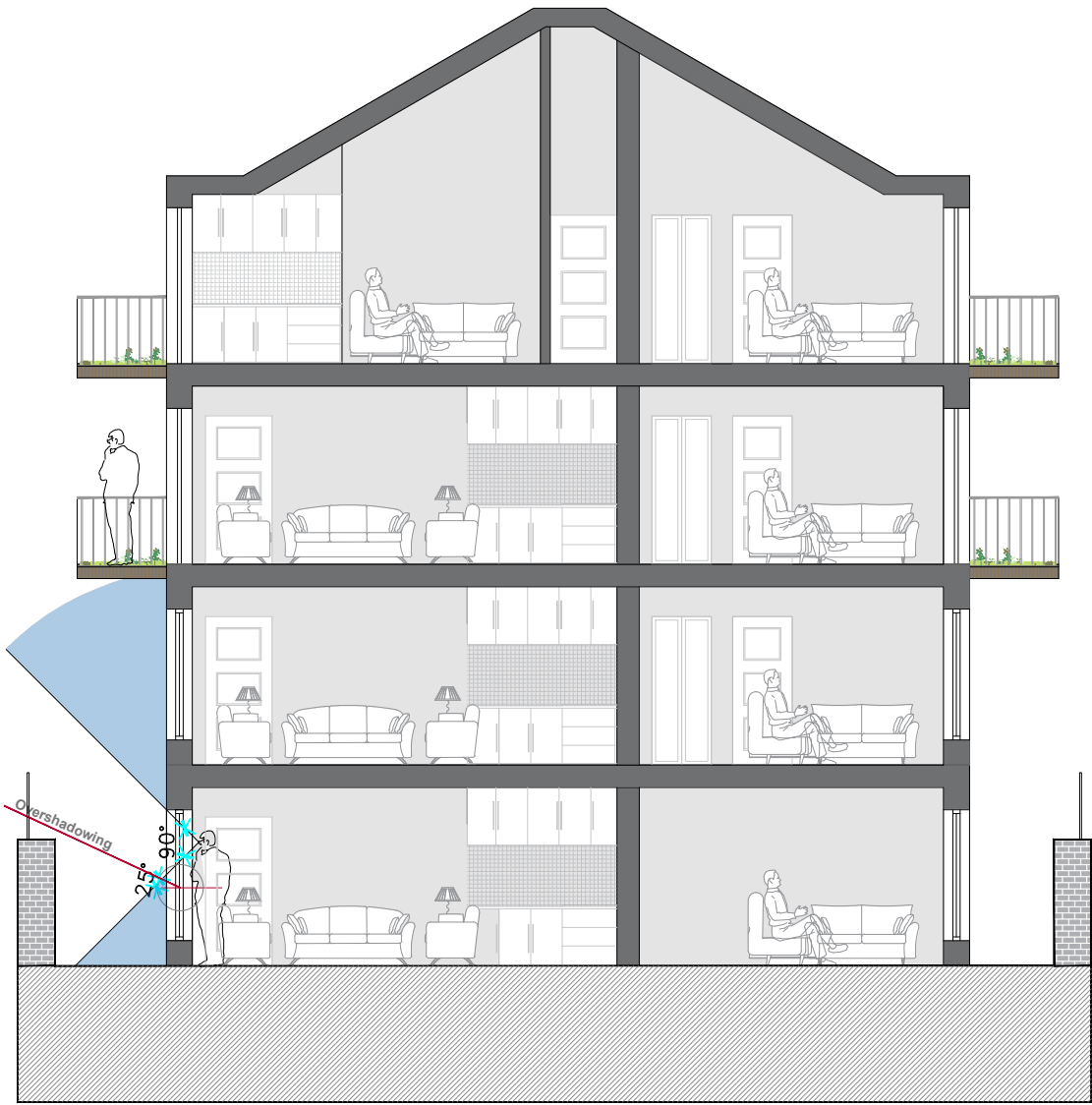
Section B-B
