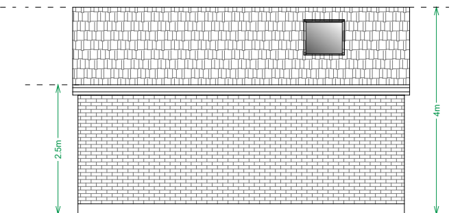
PROPOSED SIDE ELEVATION- 'B'
