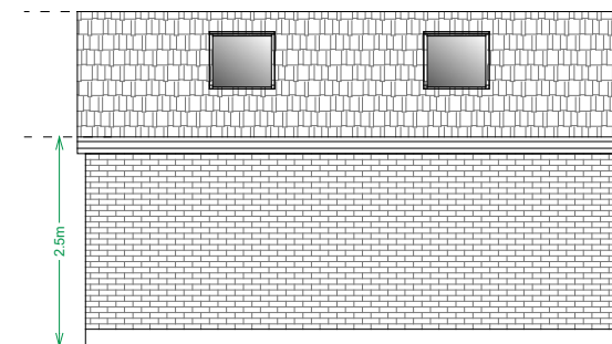
PROPOSED SIDE ELEVATION- 'A'
