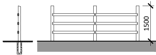
Proposed sand school fencing 1:100
