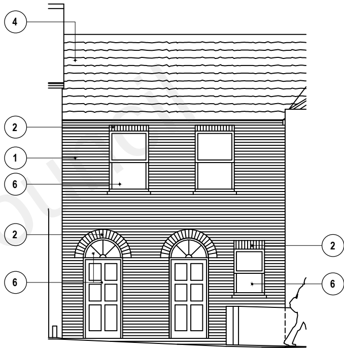
FRONT VIEW FINISHES DETAIL
