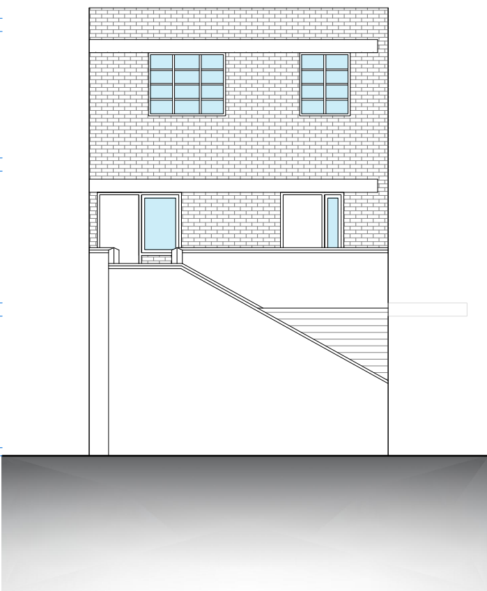
REAR ELEVATION
