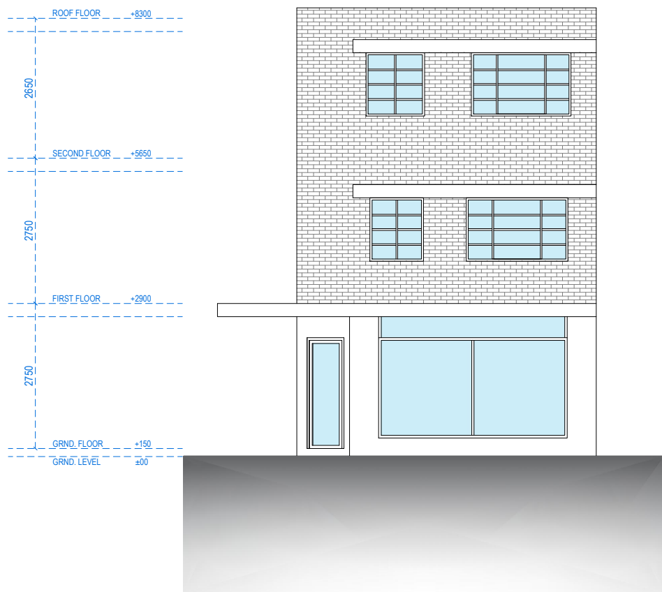
FRONT ELEVATION
