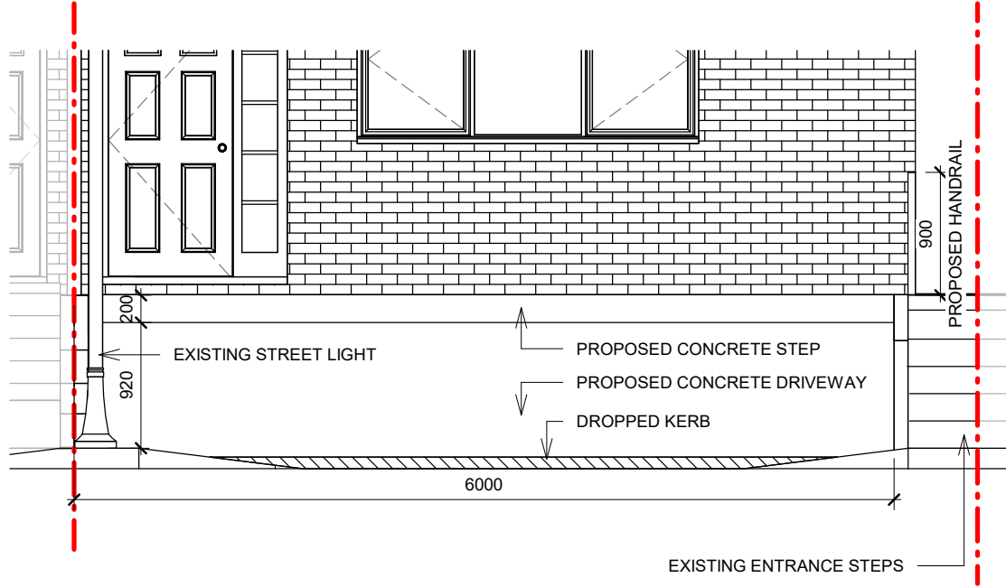
2 FRONT ELEVATION 1 : 50
