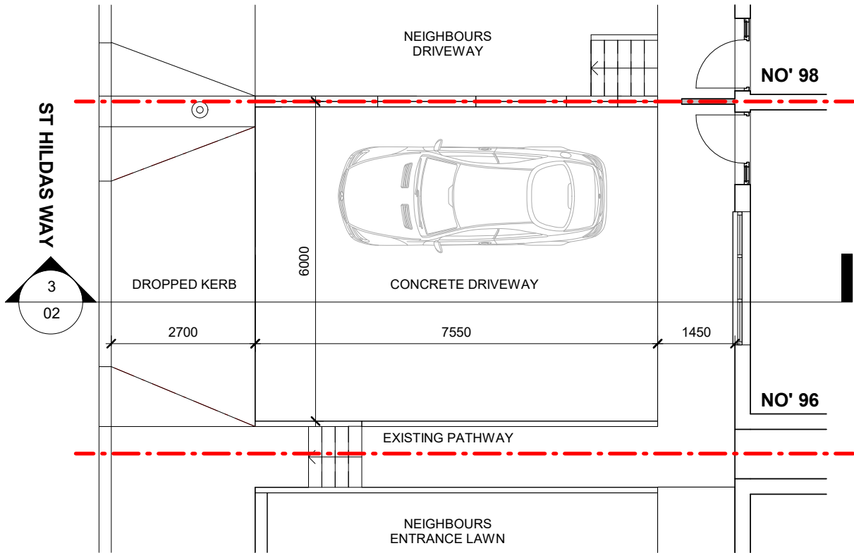
1 PROPOSED GROUND FLOOR PLAN 1 : 100
