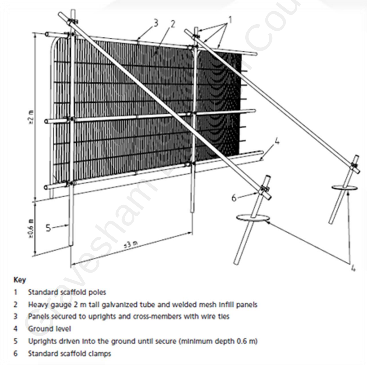
Figure 2: BS5837:2012 - Figure 2, Default specification for protective barriers.
