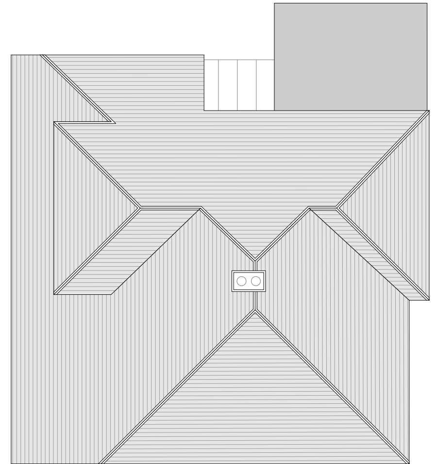
Existing Roof Plan Scale 1:100 @ A3
