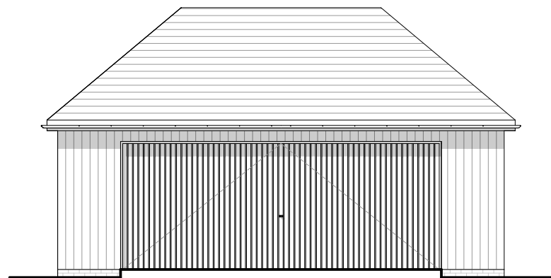
Proposed Front (South) Elevation Scale 1:100 @ A3
