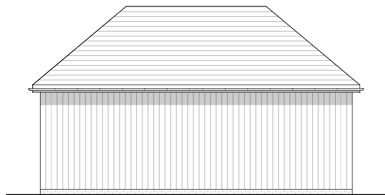
Proposed Rear (North) Elevation Scale 1:100 @ A3
