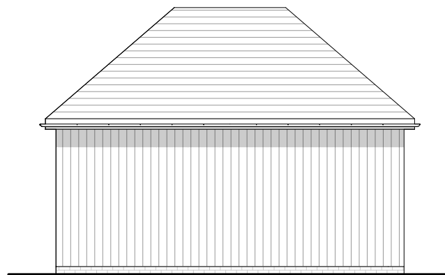
Proposed Side (West) Elevation Scale 1:100 @ A3
