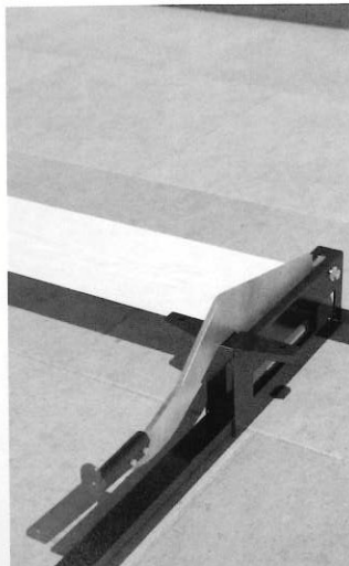
When using the Hardie™ Guillotine cutting tool, the painted face of the board must be upward facing.
