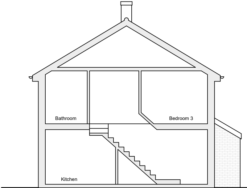
PROPOSED SIDE (North) ELEVATION / SECTION
