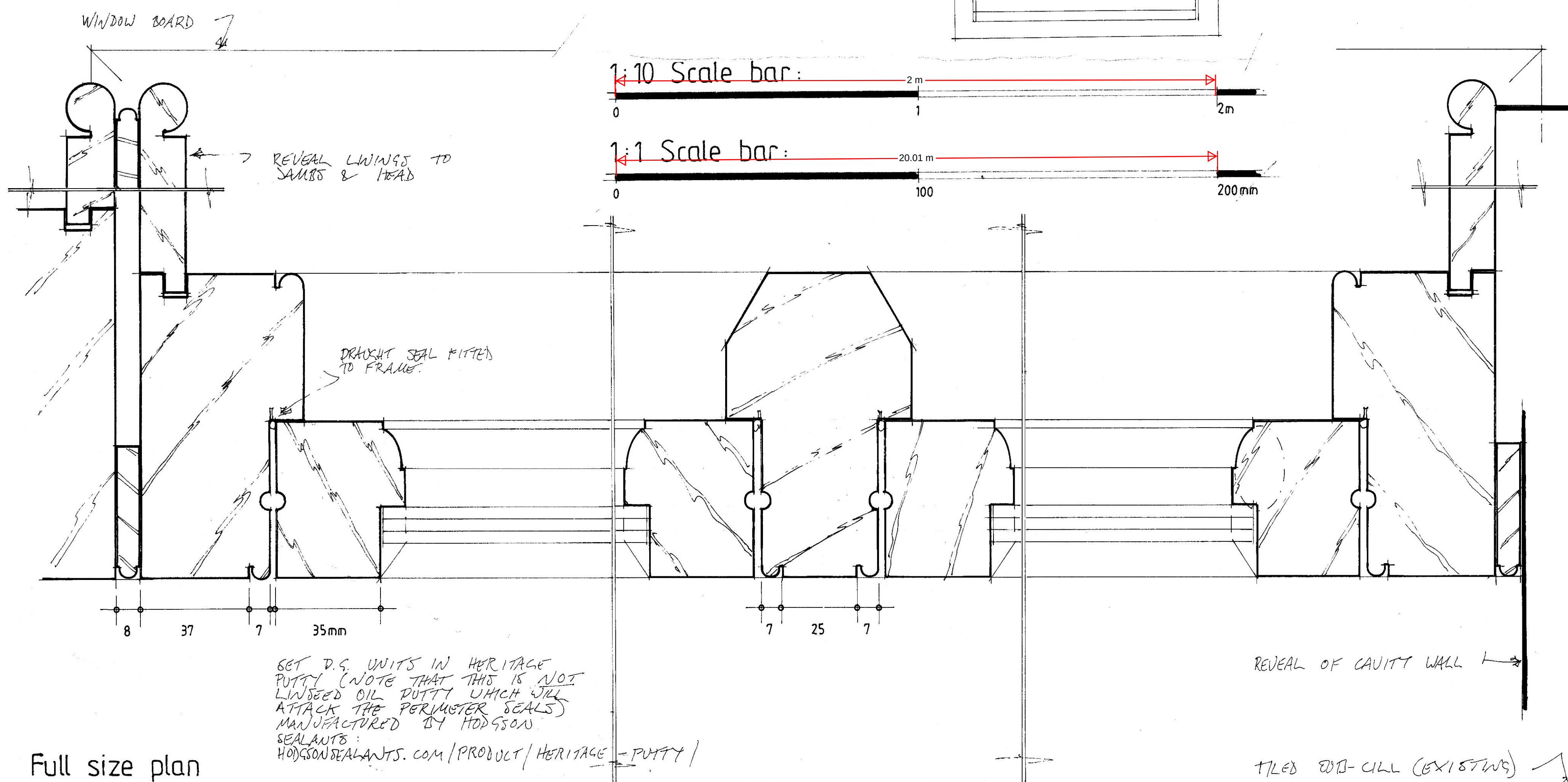
Junction between door & window frames
