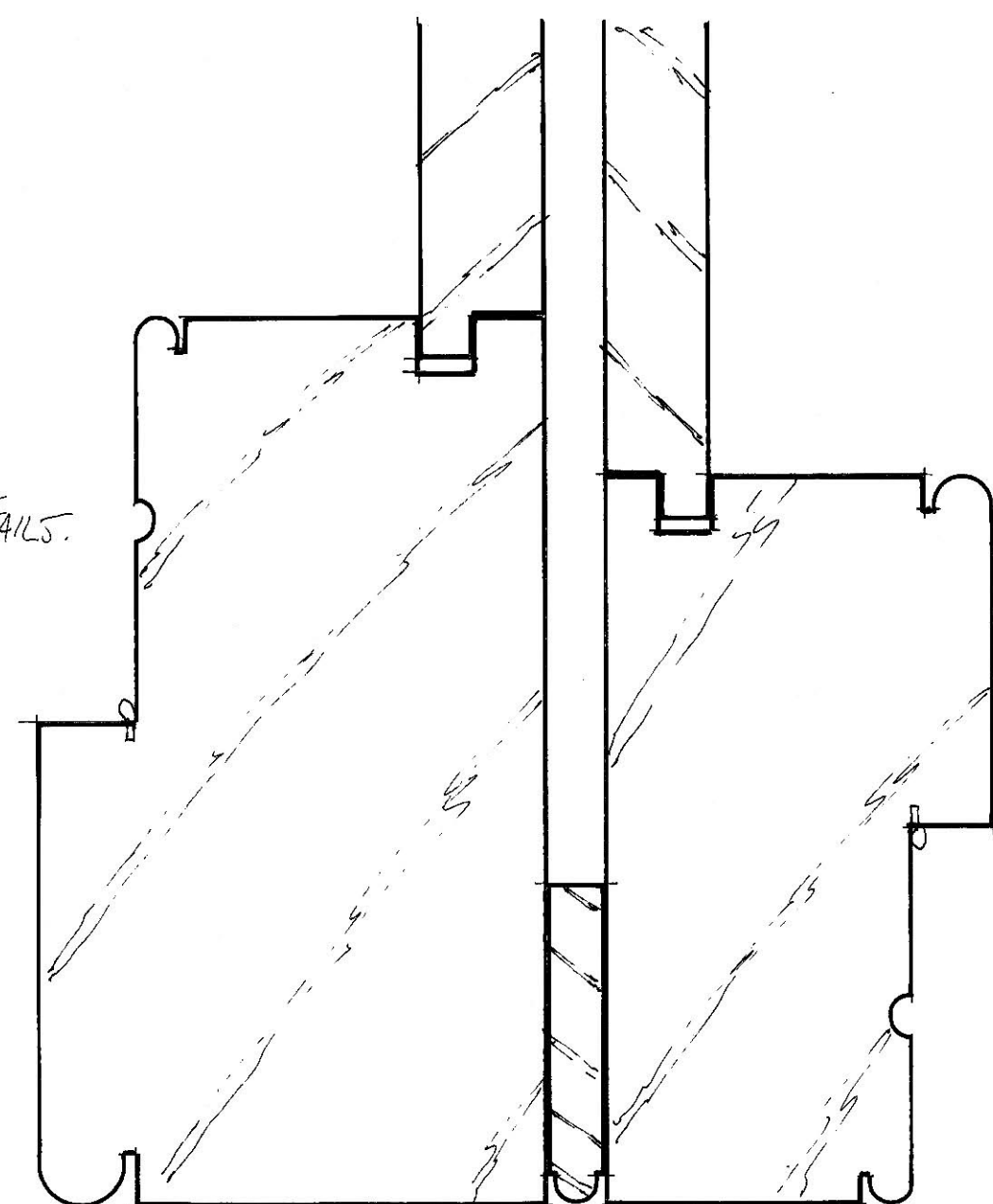
Junction between door & window frames
