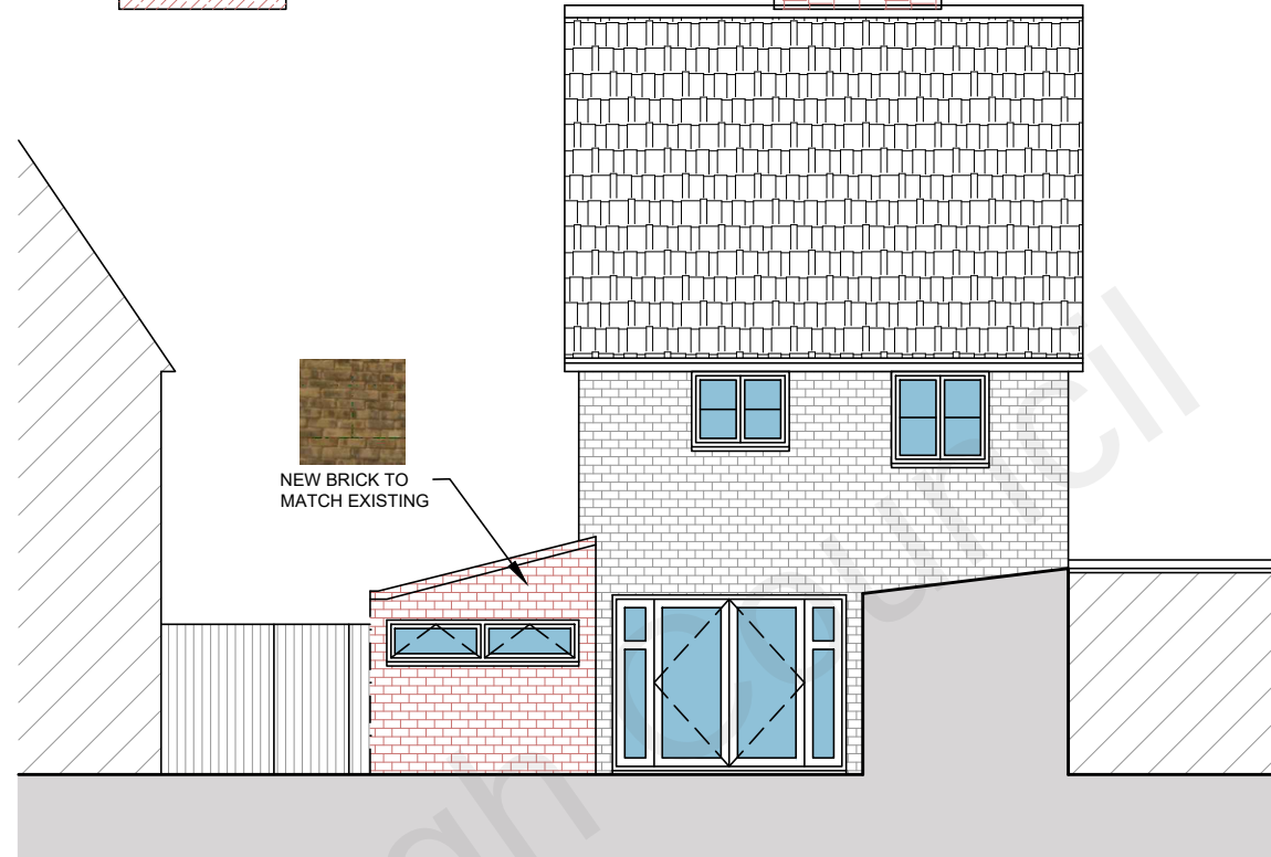
REAR ELEVATION
