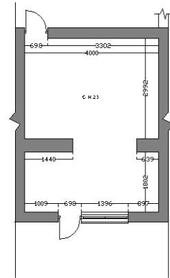
EXISTING GROUND FLOOR PLAN SCALE: 1:100
