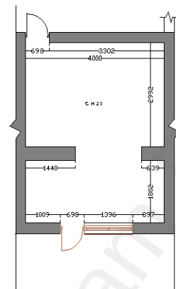
PROPOSED GROUND FLOOR PLAN SCALE: 1:100
