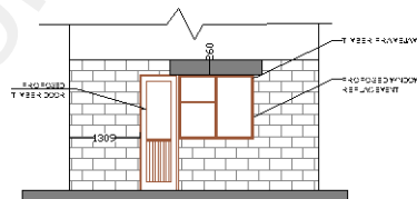
PROPOSED GROUND FLOOR REAR ELEVATION SCALE: 1:100
