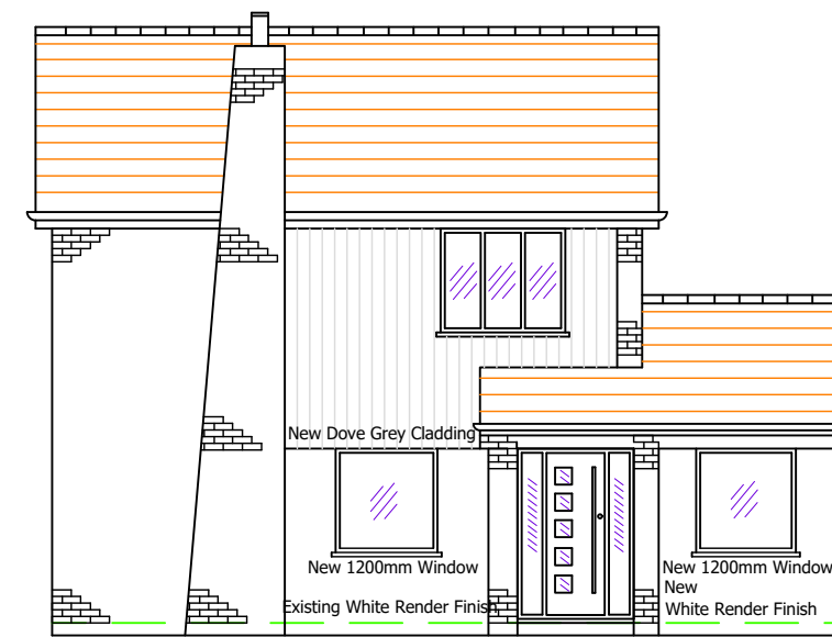
Proposed Front (North) Elevation 1:100
