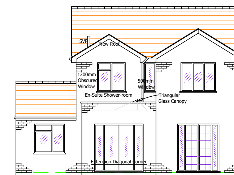
Proposed Rear (South) Elevation 1:100
