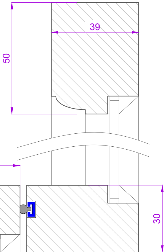
SECTION THROUGH MEETING RAIL - SCALE 1:1
