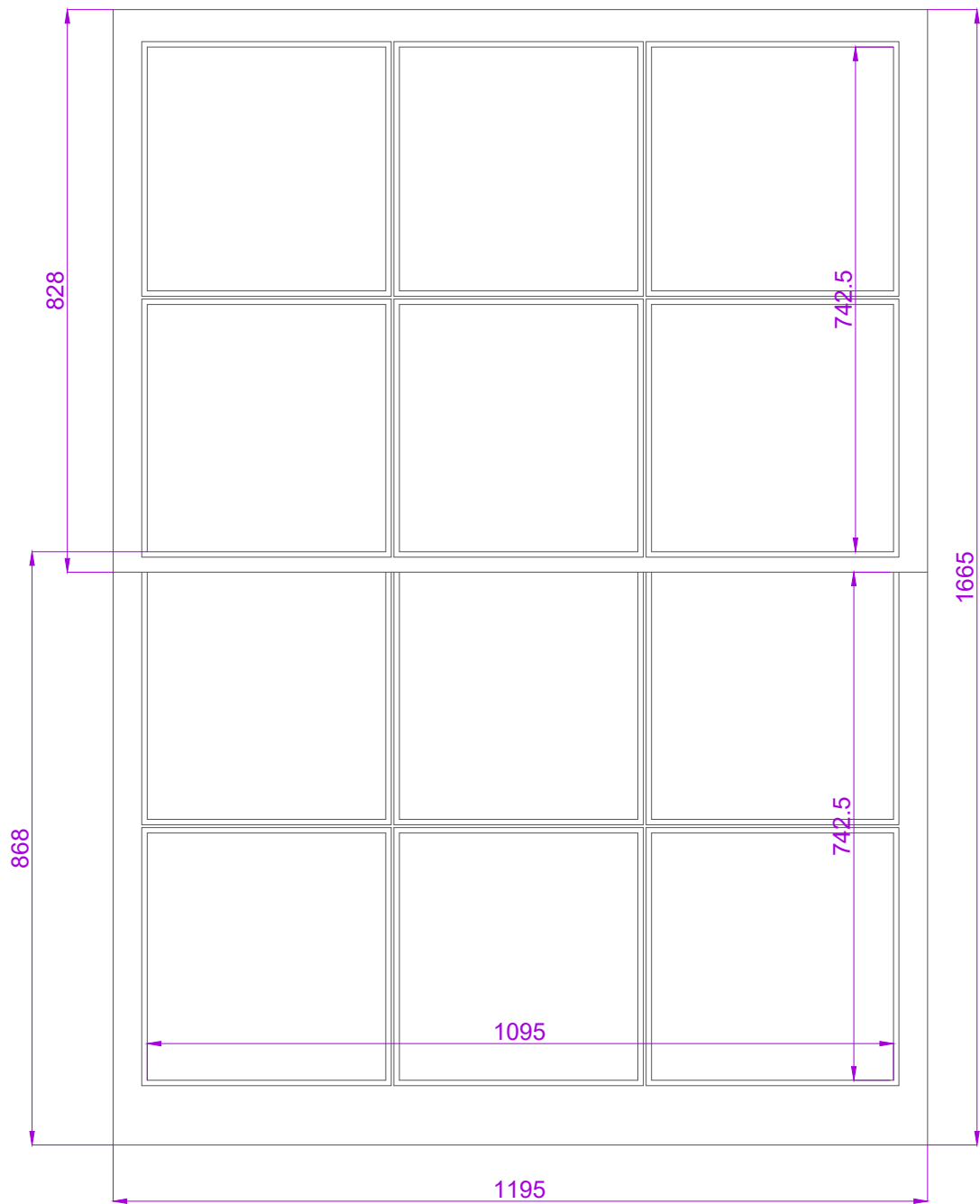
EXTERNAL VIEW - SCALE 1:10
