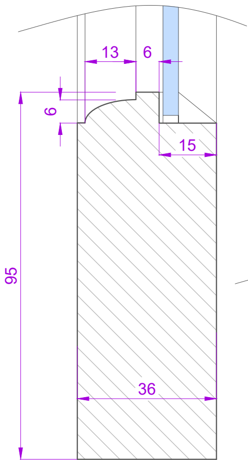
SECTION THROUGH BOTTOM RAIL - SCALE 1:1
