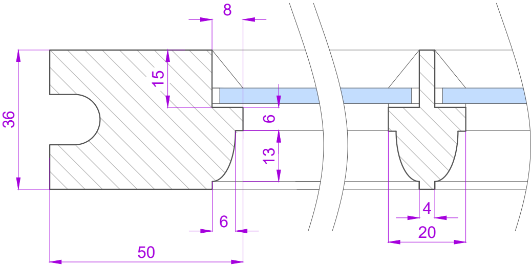
SECTION THROUGH STILE - SCALE 1:1
