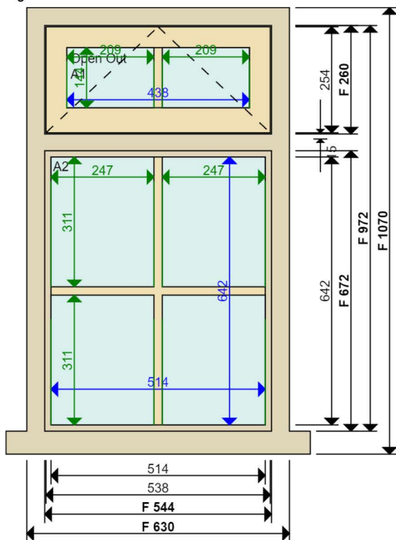
Flush casement window, Opening out, Viewed internally
