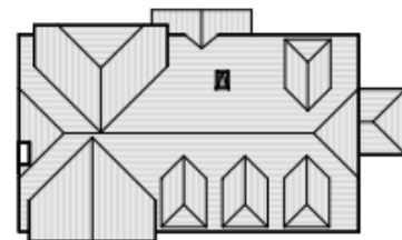
3 ROOF PLAN Scale: 1:100
