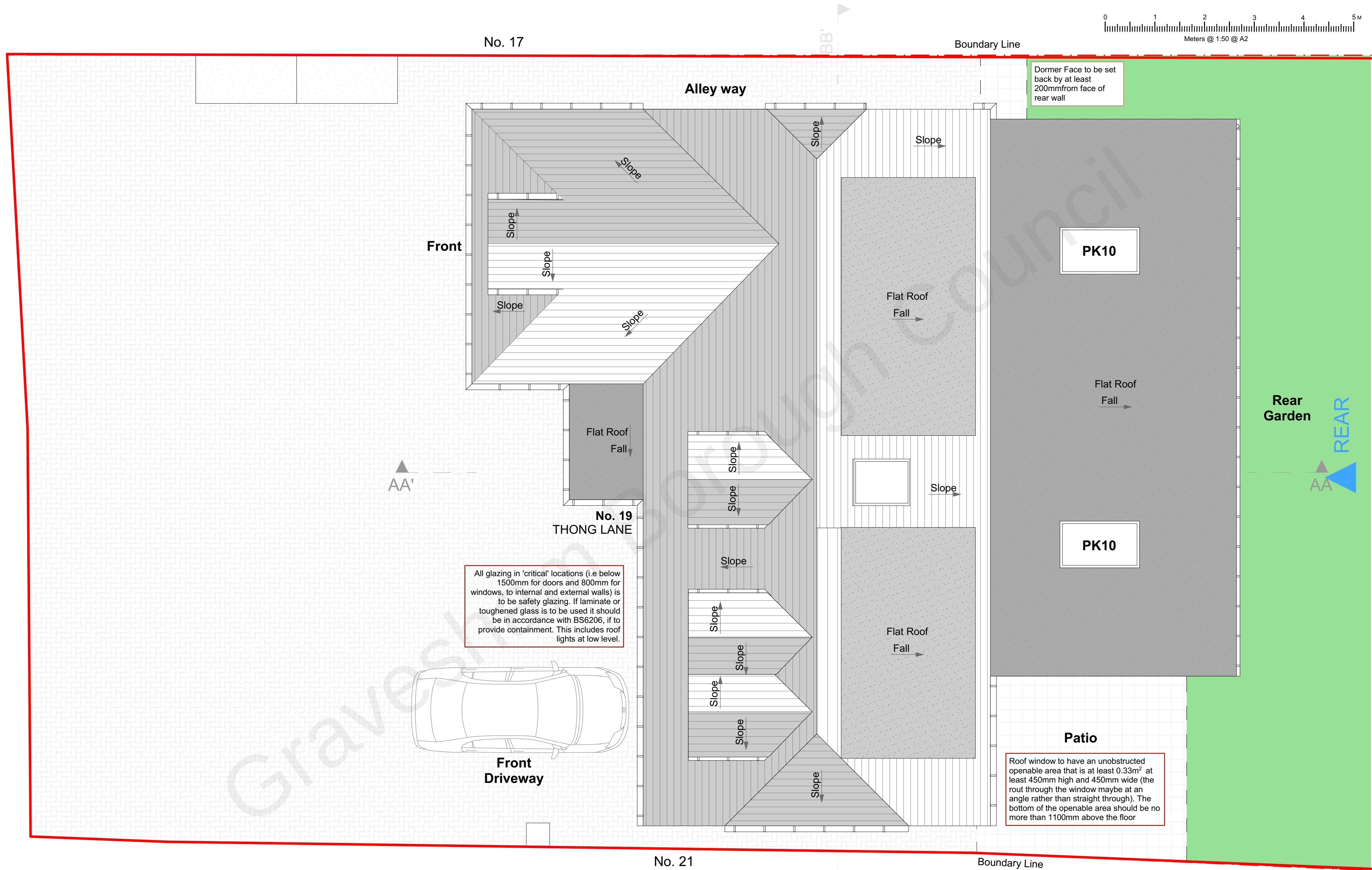
Proposed Roof Plan 1:50
