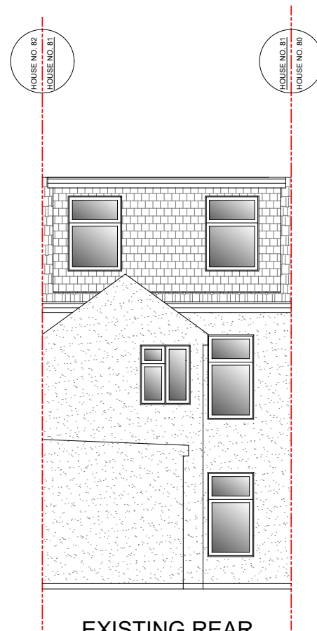
EXISTING REAR ELEVATION (no proposed changes)
