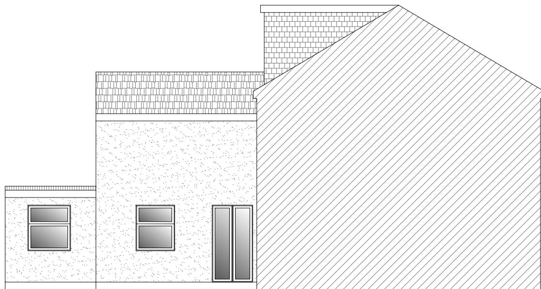
EXISTING SIDE ELEVATION- 'A' (no proposed changes)
